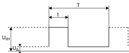
Fig. 49 Signal MLI
